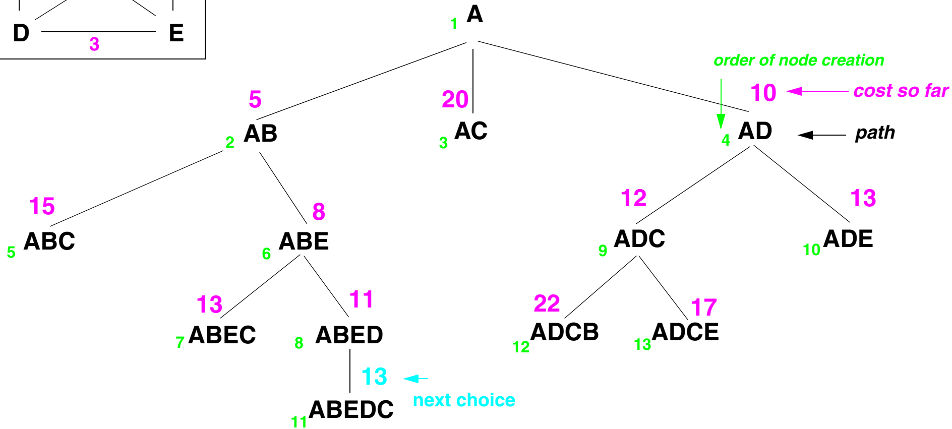
Solution space
