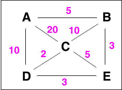
Connection graph
