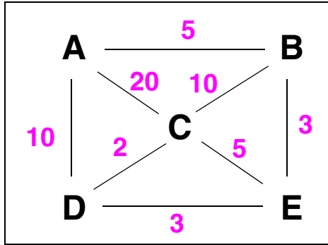
Connection graph
