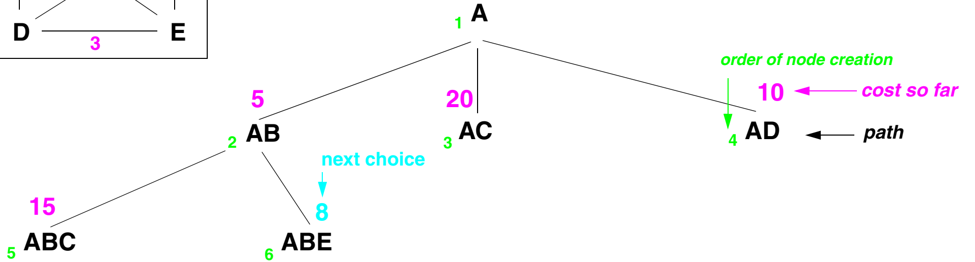
Solution space
