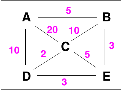
Connection graph
