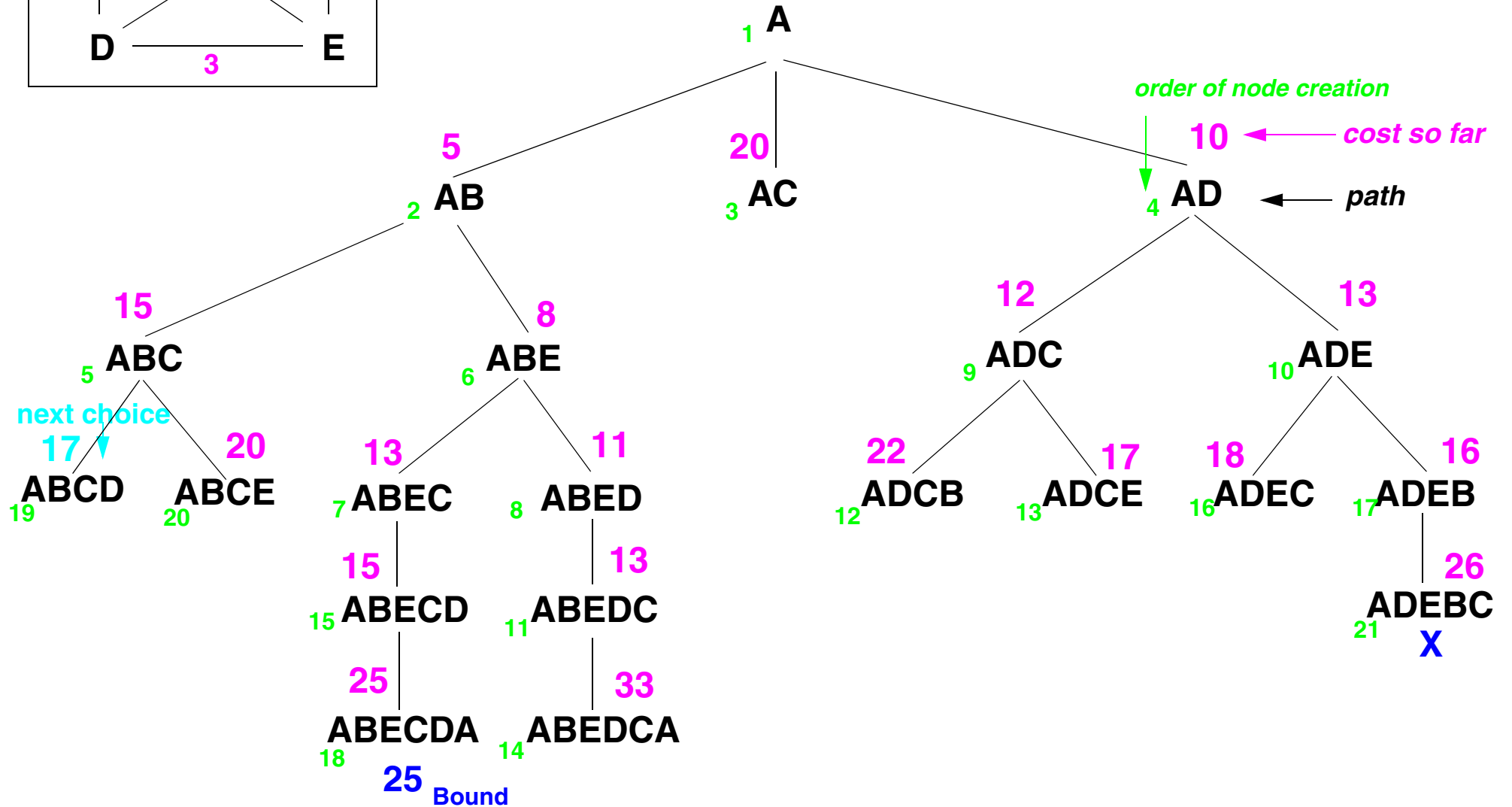
Solution space
